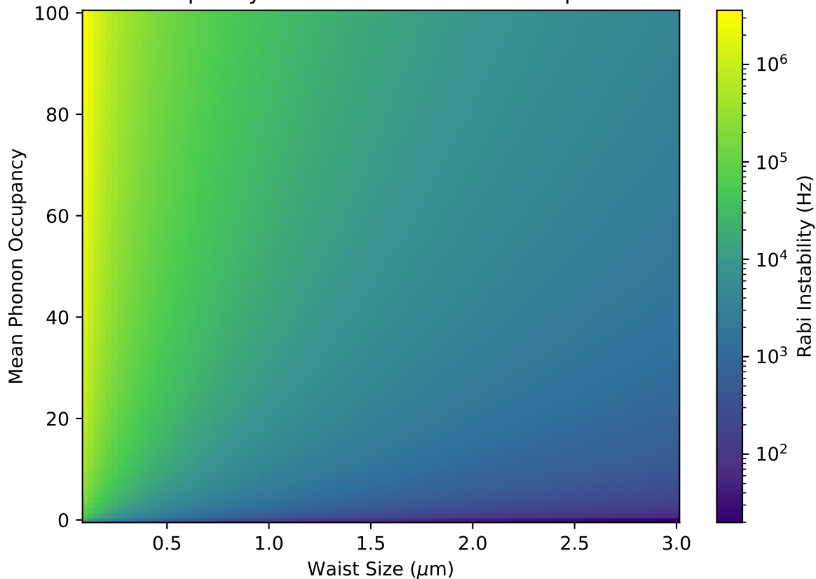
Rabi Frequency Deviation at Different Temperatures
